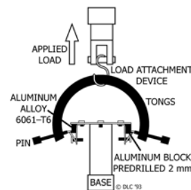
FIG. 1 Suspended Tongs
