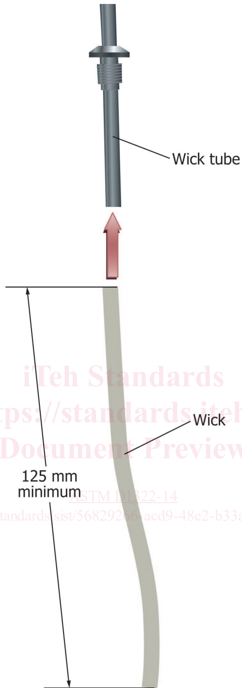
FIG. 3 Wick Tube
