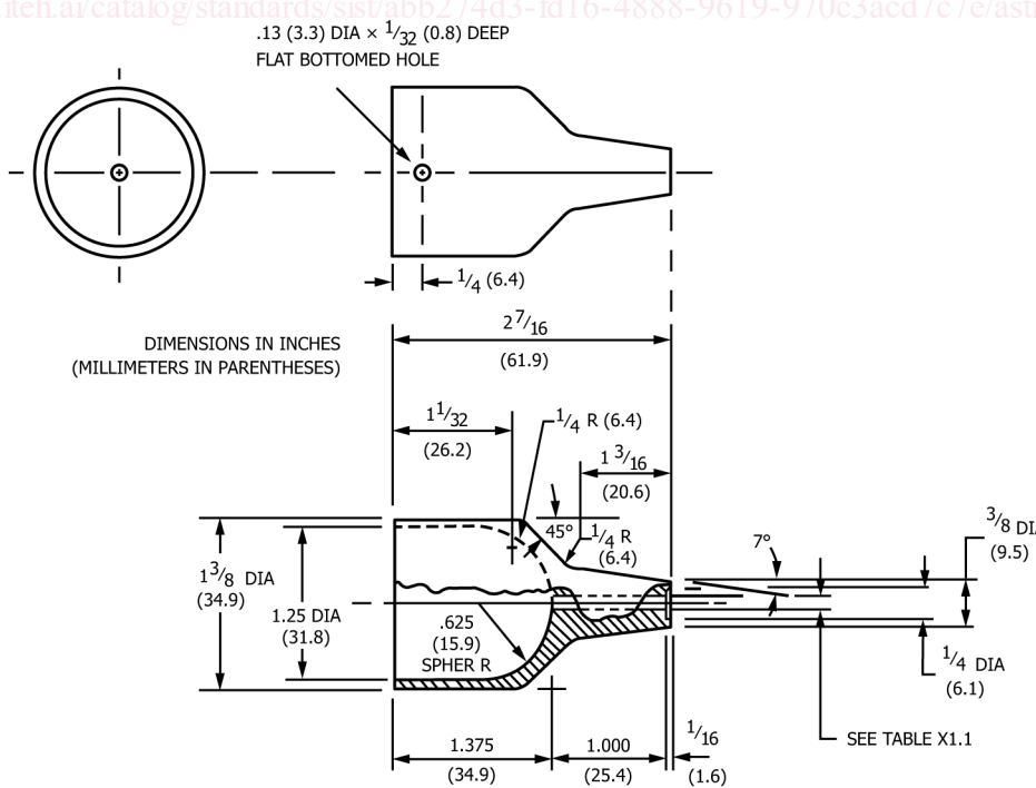
FIG. 2 Shell Cup
