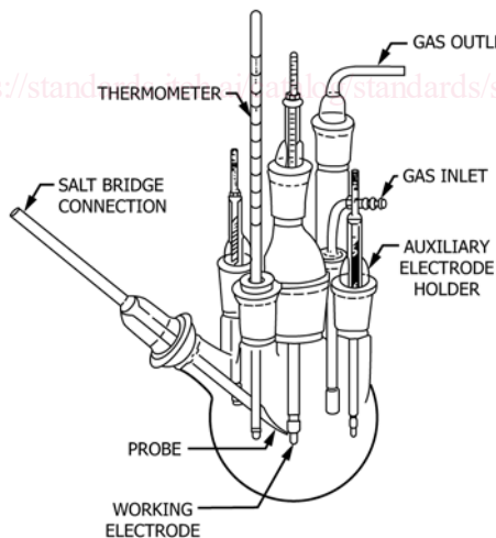
FIG. 2 Schematic Diagram of Polarization Cell (1)
