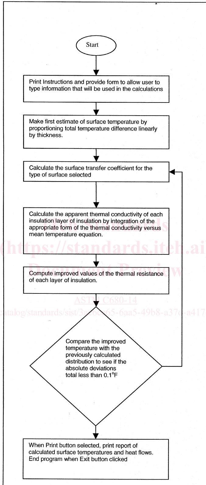
FIG. 1 Flow Chart
