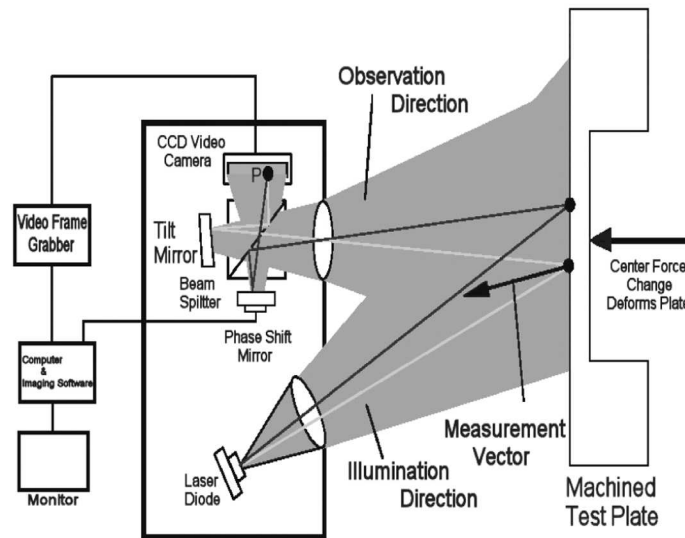
FIG. 21 Schematic diagram of a Michelson type shearing interferometer shown with a shearography calibration device consisting of a metal plate with a machined flat bottomed hole creating a deformable plate with a precision mechanical mechanism for loading at the center point.
