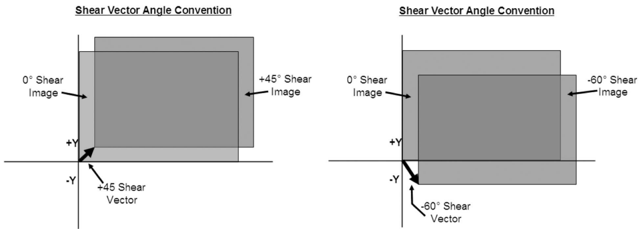
FIG. 12 Shear vector angle convention: Starting with the shear camera adjusted for a 0° shear condition, the sheared image is moved to the right (+X) or up/down, never adjusted in the direction of -X. For a +45° shear vector, the image is moved in the +X and +Y direction. For 60° shear vector, the image is adjusted in the +X and -Y directions. The convention allows determination of deformation direction from the unwrapped phase map.
