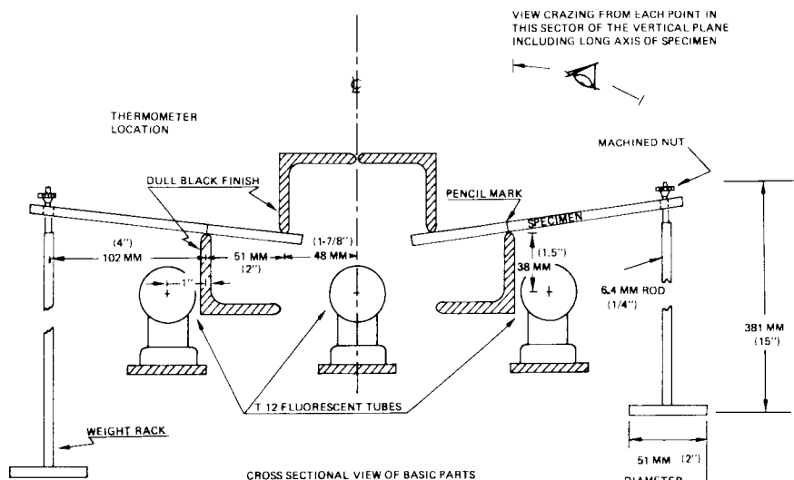
FIG. 1 Accelerated Craze Test Fixture
