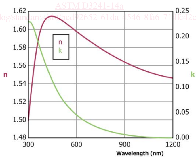
FIG. A2.4 n and K Values of the Heater Tube
