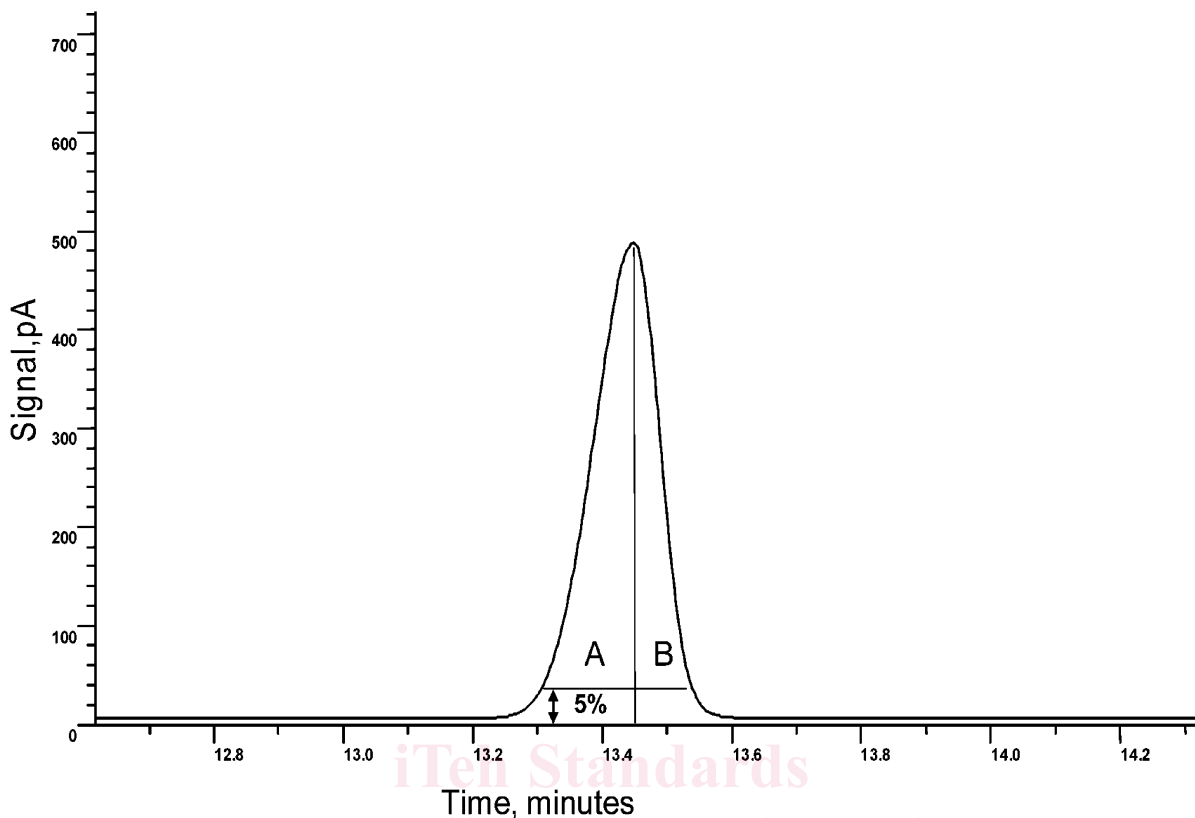
FIG. 3 Peak Skewness for Calibration Mix Peak C 20
