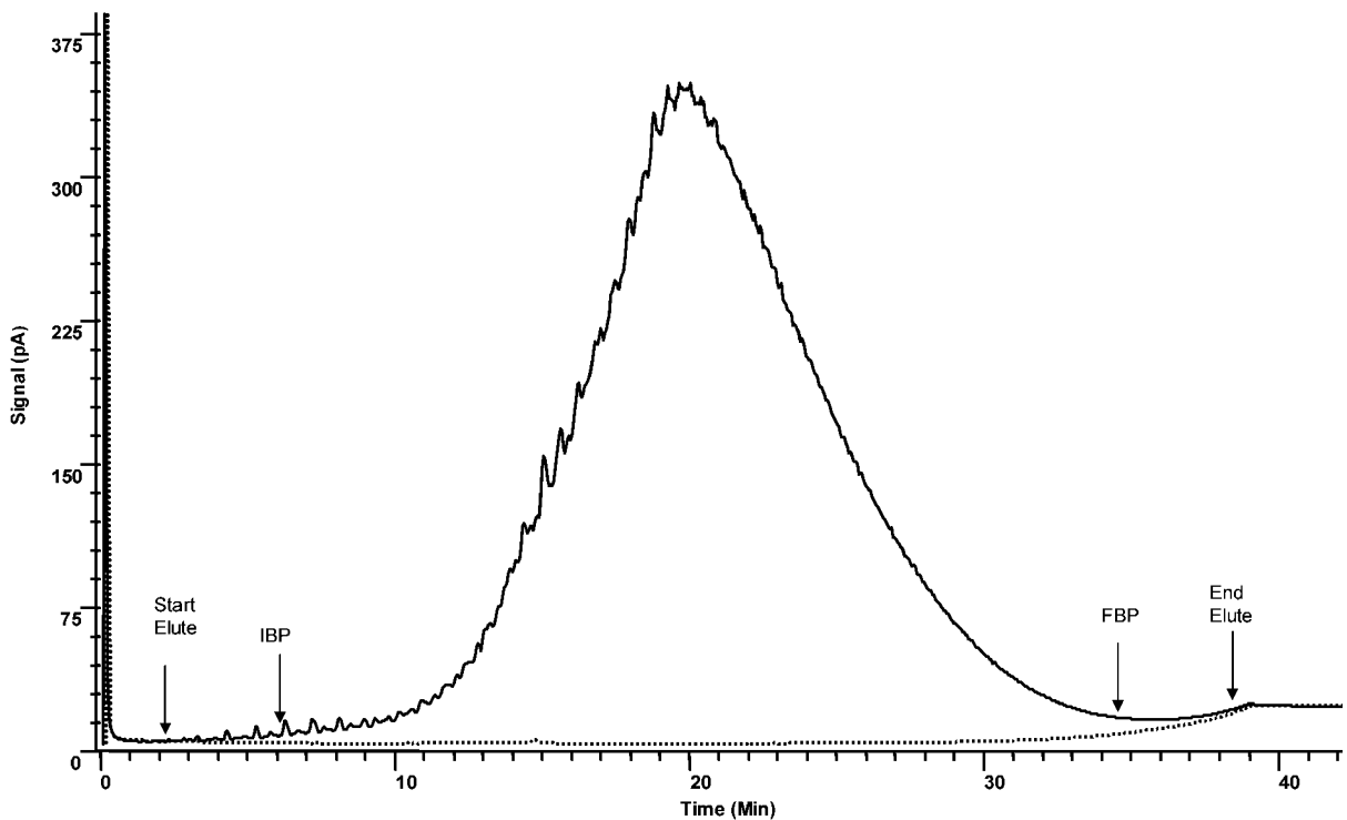
FIG. 1 Typical Sample Chromatogram which has a FBP of 700°C/700 °C
