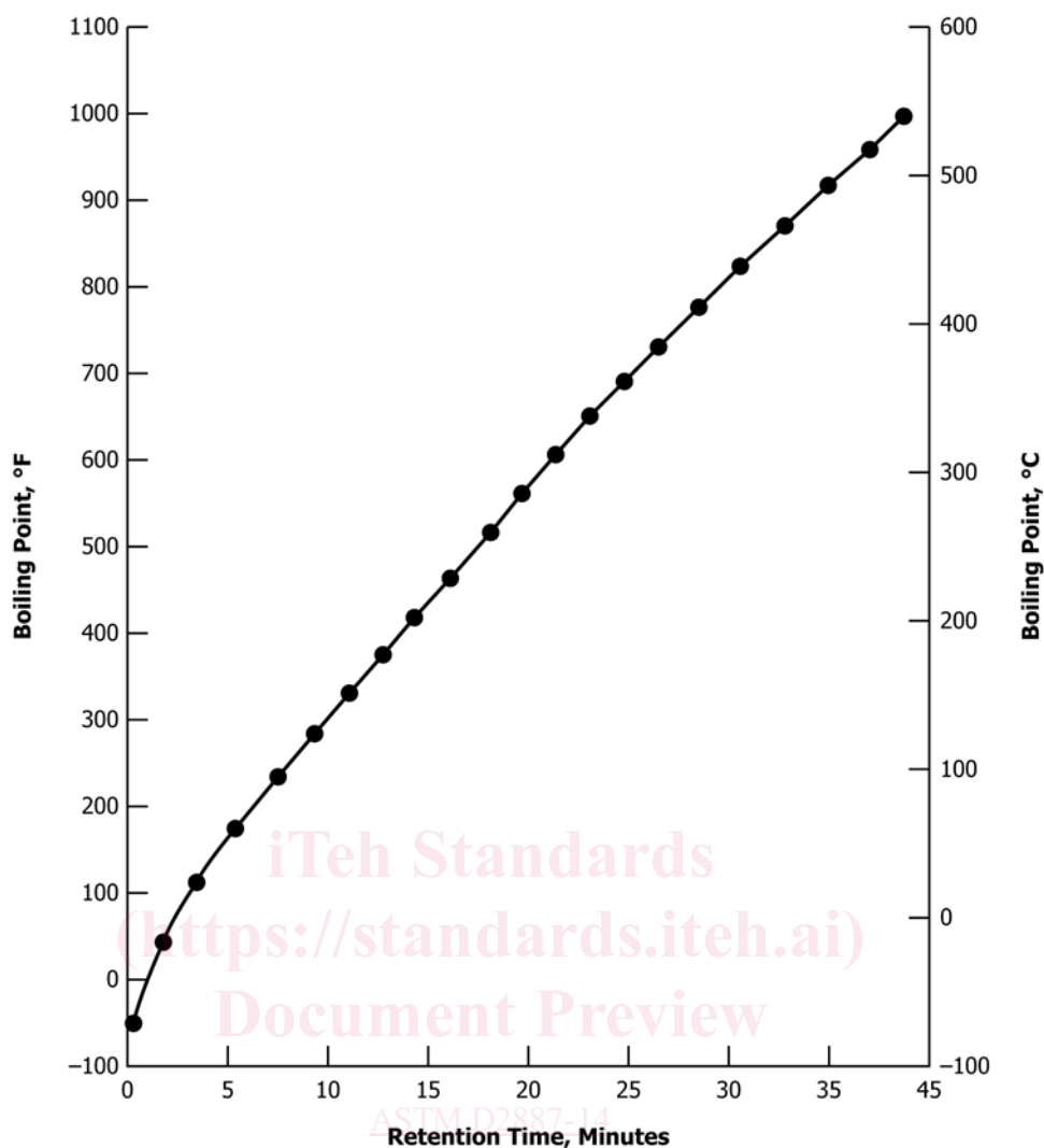
ASTM D2887-14 FIG. 2 Typical Calibration Curve
