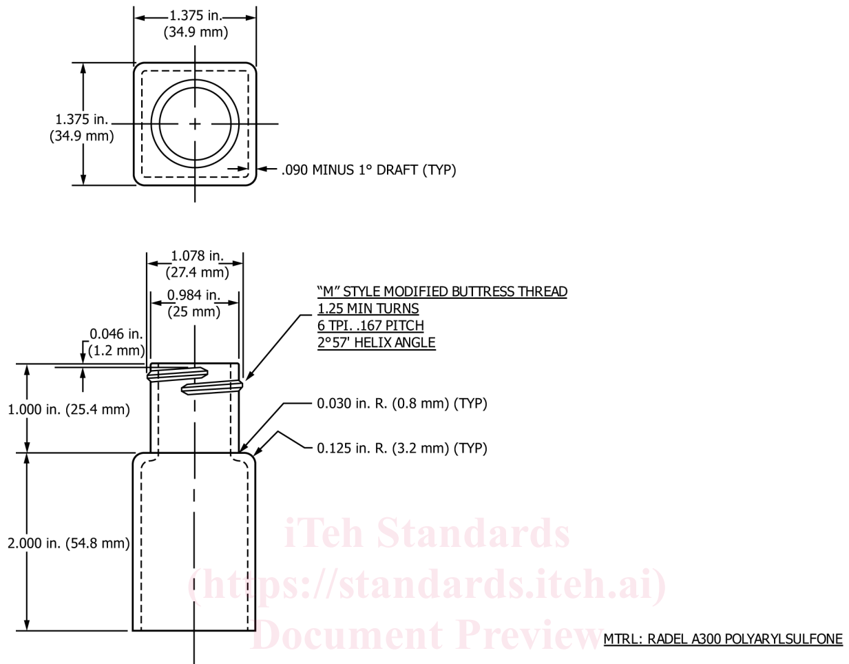
FIG. 1 Typical Fixture
