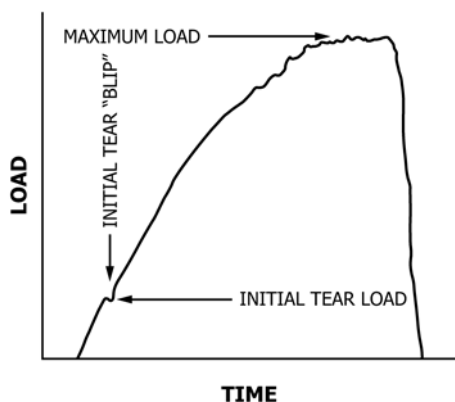
FIG. 2 Load-Time Chart for Highly Extensible Film
