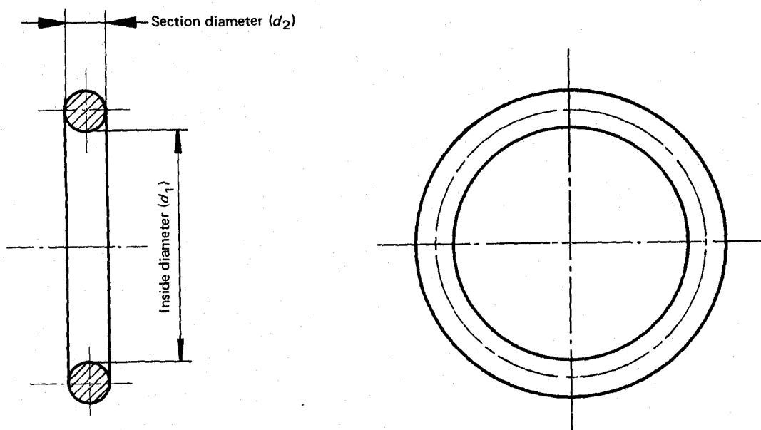
FIGURE – Typical O-ring
