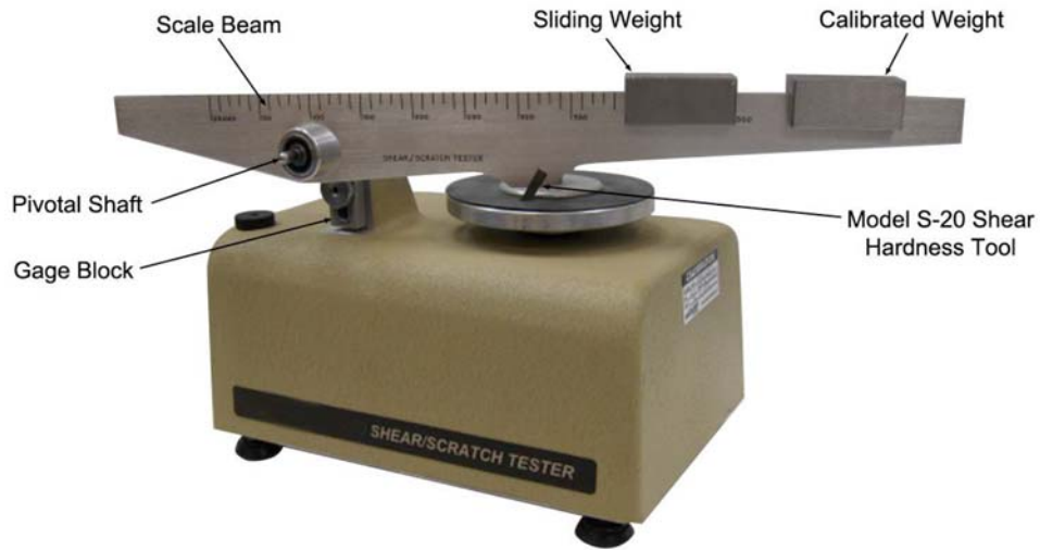
FIG. 1 Shear/Scratch Tester
