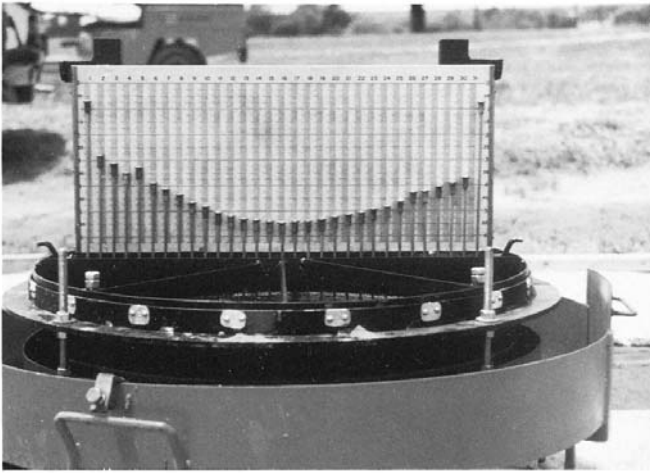
FIG. 3 Pin Profile Following a Time Sequence
