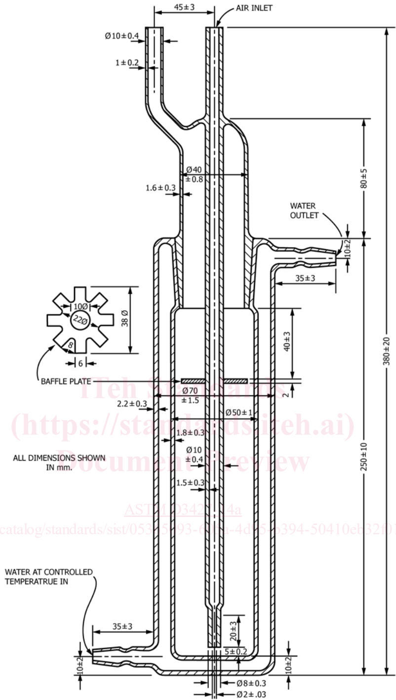
FIG. 2 Test Vessel
