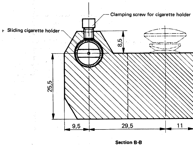
FIGURE 2 — Direct method — Details of cigarette holder
