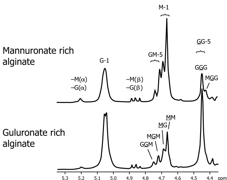
FIG. 12 Typical 1 H NMR of Sodium Alginate
