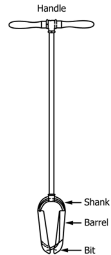
FIG. 3 Post-Hole Type (Iwan-type) Barrel Auger
