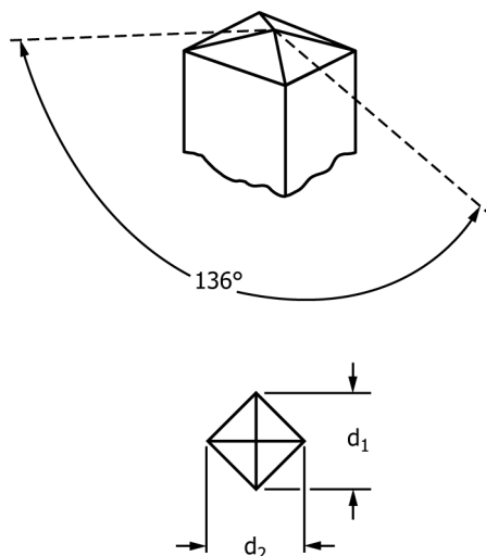
FIG. 12 Vickers Indenter
