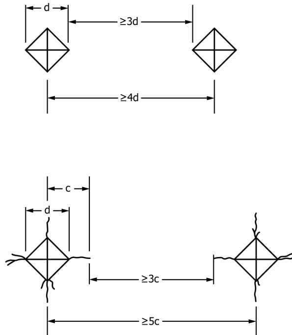
FIG. 23 Closest Permitted Spacing for Vickers Indentations
