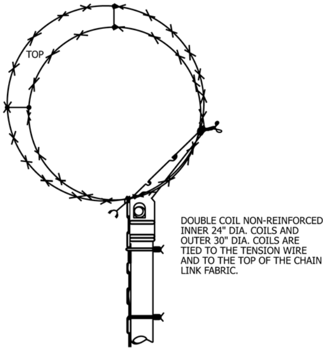
FIG. 5 Top of the Fence 45° Barb Arm Installation
