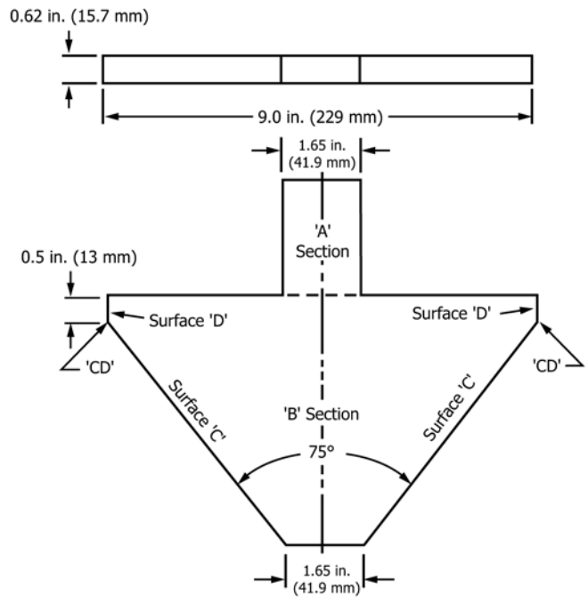
FIG. 4 Test Probe for Partially Bounded Openings
