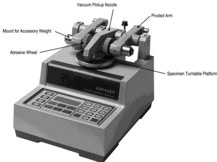
FIG. 1 Rotary Platform, Double-Head (RPDH) Abraser, with Dual Testing Platforms Platform Abraser
