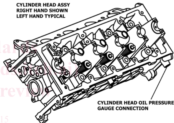
FIG. 5 Oil Pressure Gage Connections -15
