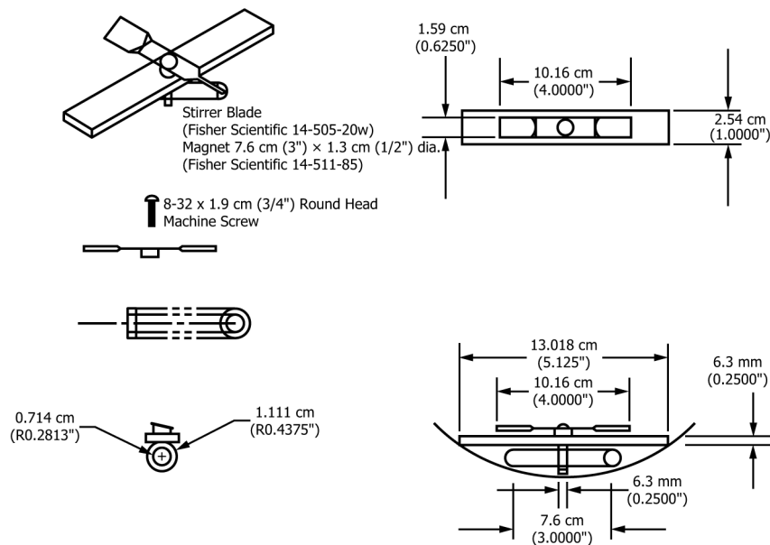
FIG. 2 Magnetic Driven Stirrer
