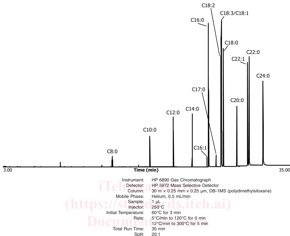
FIG. 1 Total Ion Chromatogram (TIC) of a FAME Reference Mixture on a DB-1MS Capillary Column Using Test Method E1618 GC-MS Conditions https://standards.iteh.ai/catalog/standards/sist/3bc1561b-16b9-4479-8ba8-a5fb07640937/astm-e2881-13e1
