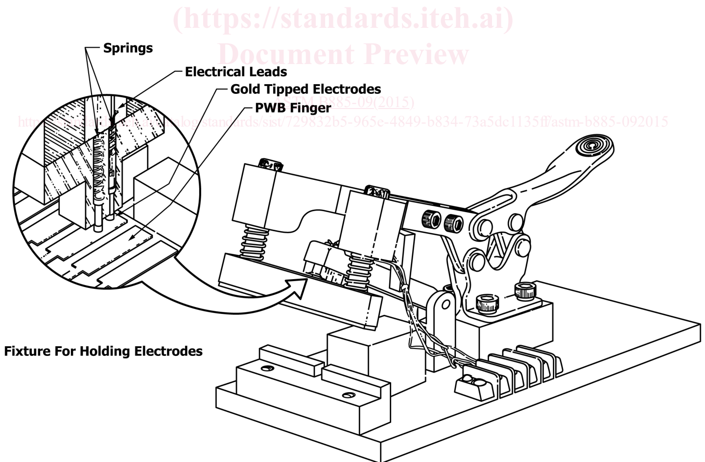
FIG. 1 Resistance Probe
