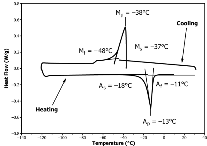
FIG. 1 DSC Graph for a Single-Stage Transformation
