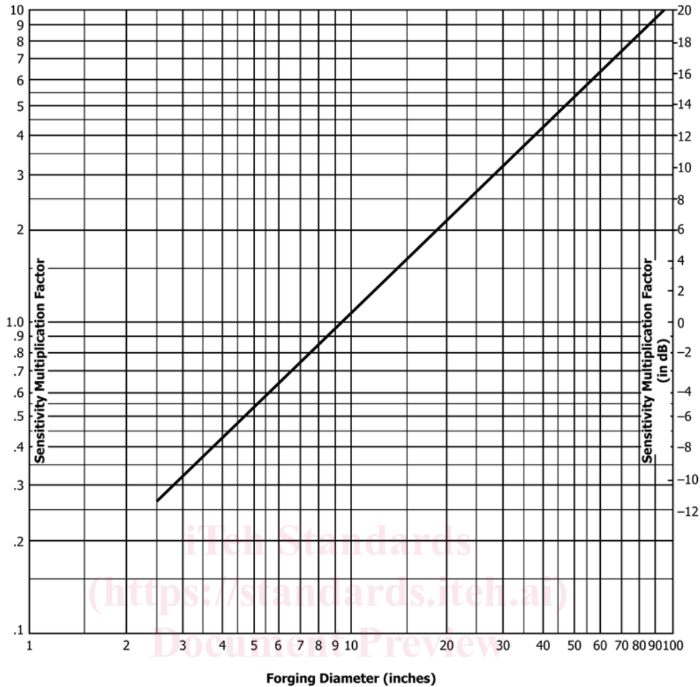
ASTM A418/A418M 15 SENSITIVITY MULTIPLICATION FACTORS FOR SOLID FORGINGS
