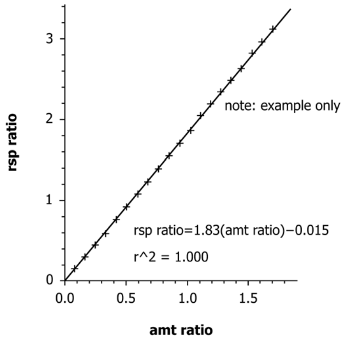
FIG. 3 A Least-Squares Fit Calibration for MTBE
