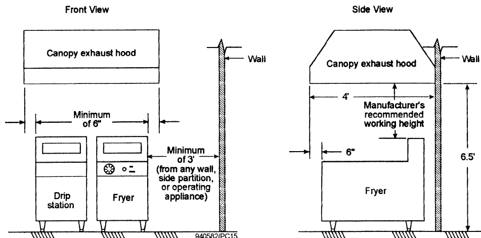
FIG. 1 Equipment Configuration
