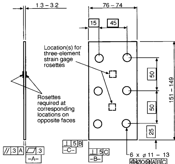
FIG. 6 Procedure A, Two-Rail Shear Specimen, SI Units
