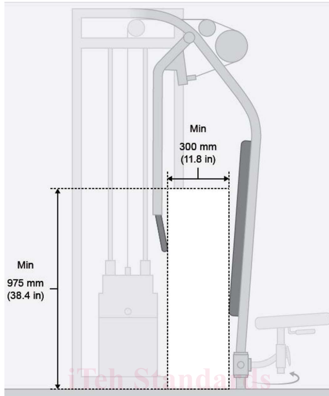
FIG. 78 Minimum Distance from Back Support to Hand Grips with Seat Removed
