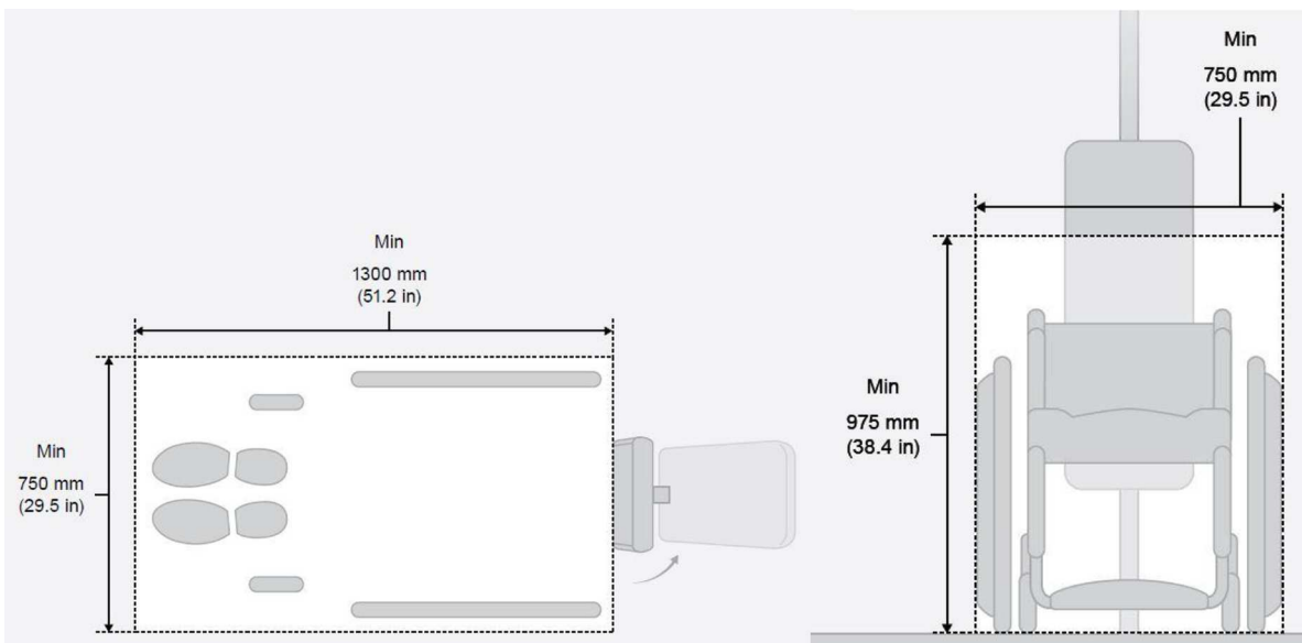
FIG. 67 Removable/Movable Minimum Clear Space Area
