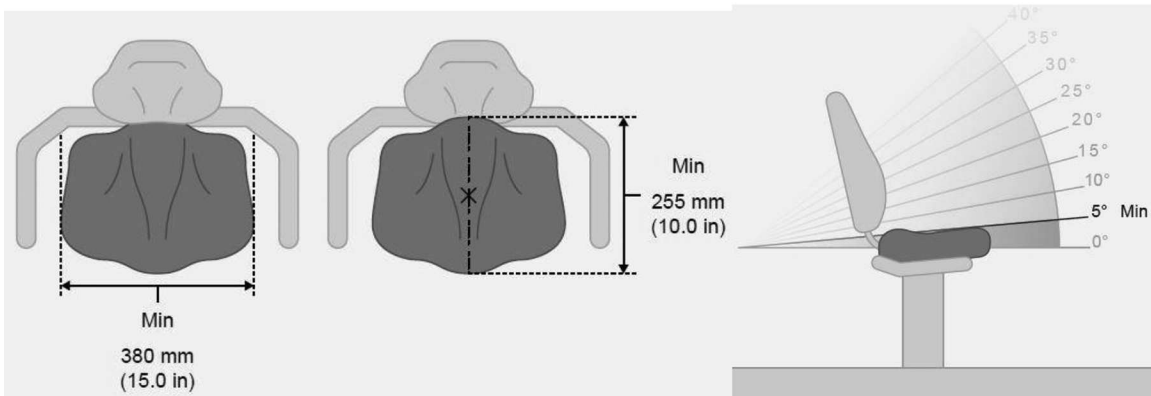
FIG. 45 Minimum Seat Dimensions – Width, Depth, Angle
