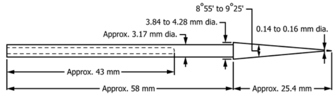
FIG. 2 Standard Needle
