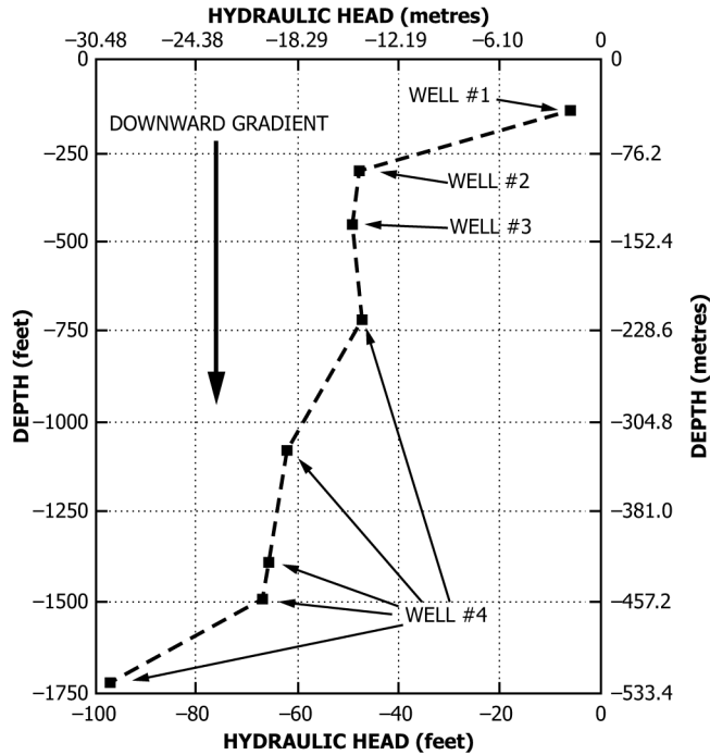
FIG. 2 Hydraulic Gradient at a Groundwater Location (data from four wells) (adapted from Ref (96))
