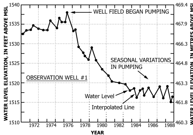
FIG. 3 Example of Simple Hydrograph (adapted from Ref (117))
