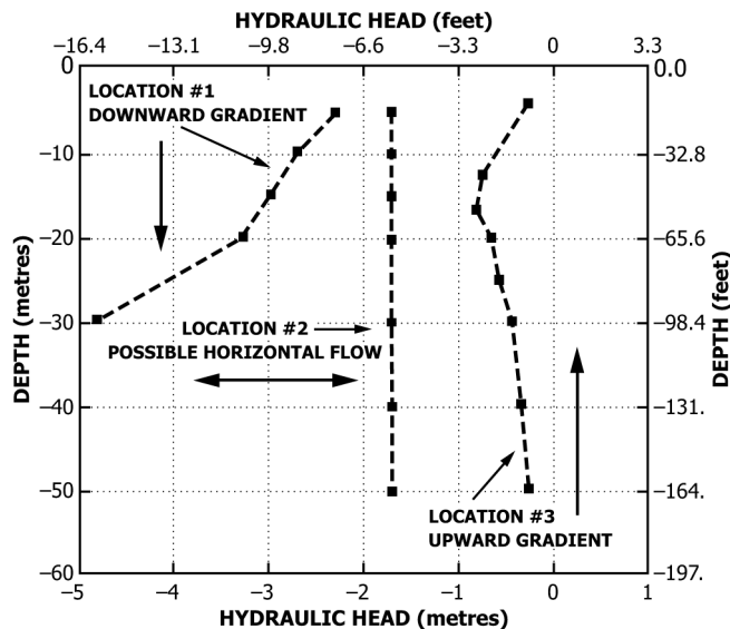
FIG. 1 Hydraulic Gradient at Three Groundwater Locations (adapted from Ref (85))
