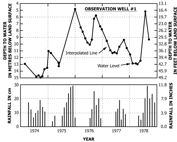
FIG. 4 Hydrograph and Precipitation Plot (adapted from Ref (148))
