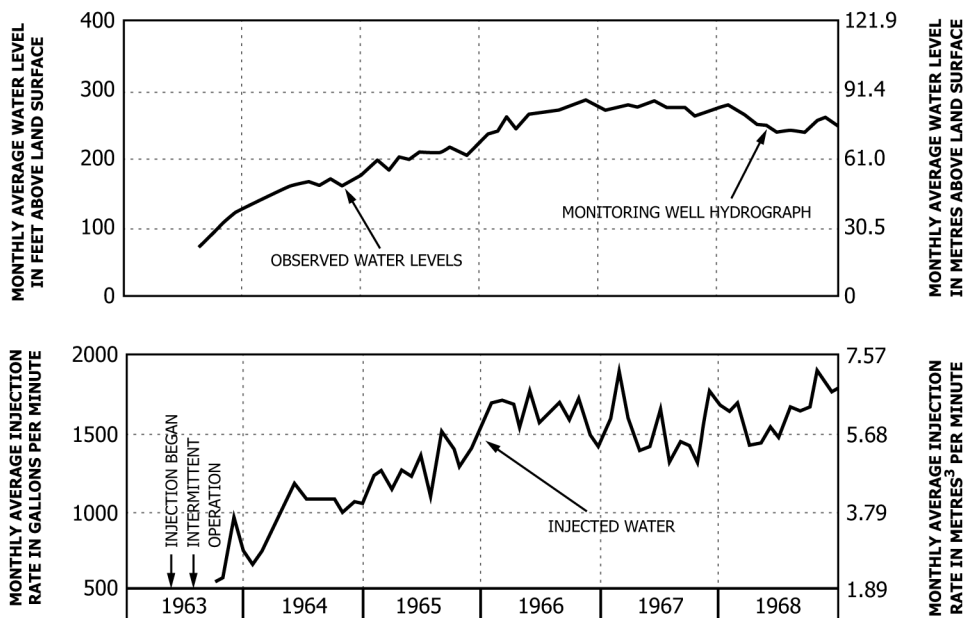
FIG. 5 Hydrograph Showing Effects of Artificial Recharge by Injection Well (adapted from Ref (179))
