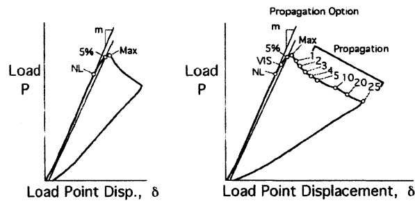
FIG. 4 Load-Displacement Curves
