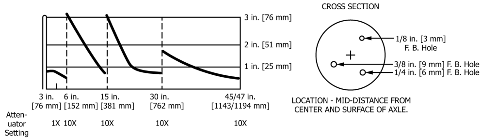
FIG. 2 Location of Reference Holes in an Axle—Flat Bottom Hole Sizes for a Heat-Treated Axle
