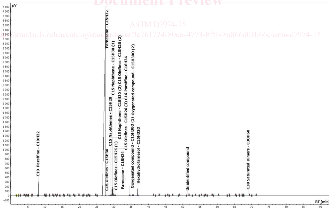
FIG. 1 Chromatogram of a Reference Distillated Farnesane
