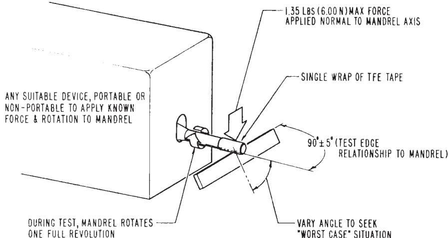
FIG. 8 Principle of Sharp Edge Test
