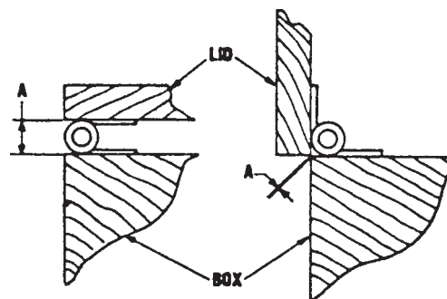
FIG. 4 Changing Clearance at Hinge Line
