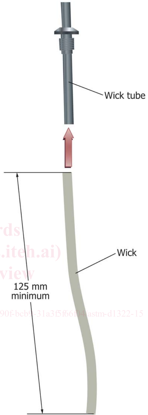
FIG. 3 Wick Tube
