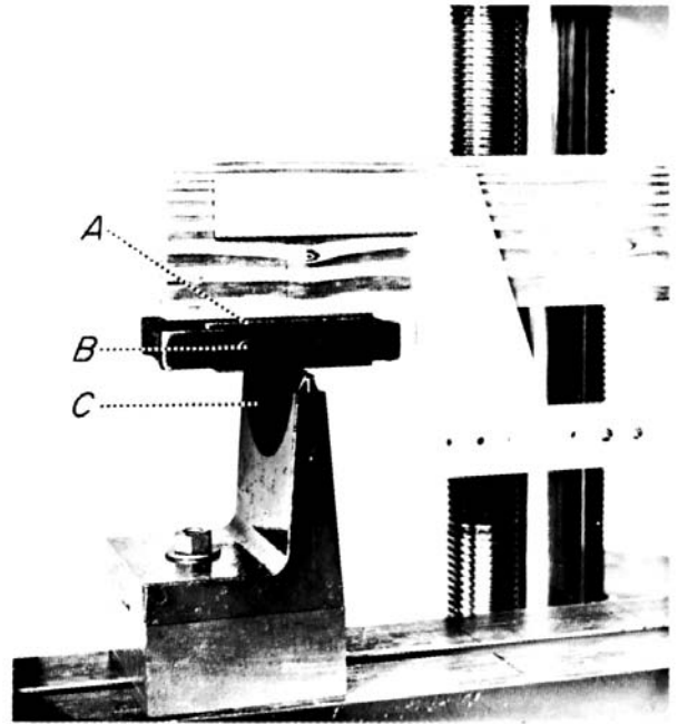
FIG. 2 Example of Bearing Plate (A), Rollers (B), and Reaction-Alignment-Rocker (C), for Small Beams
