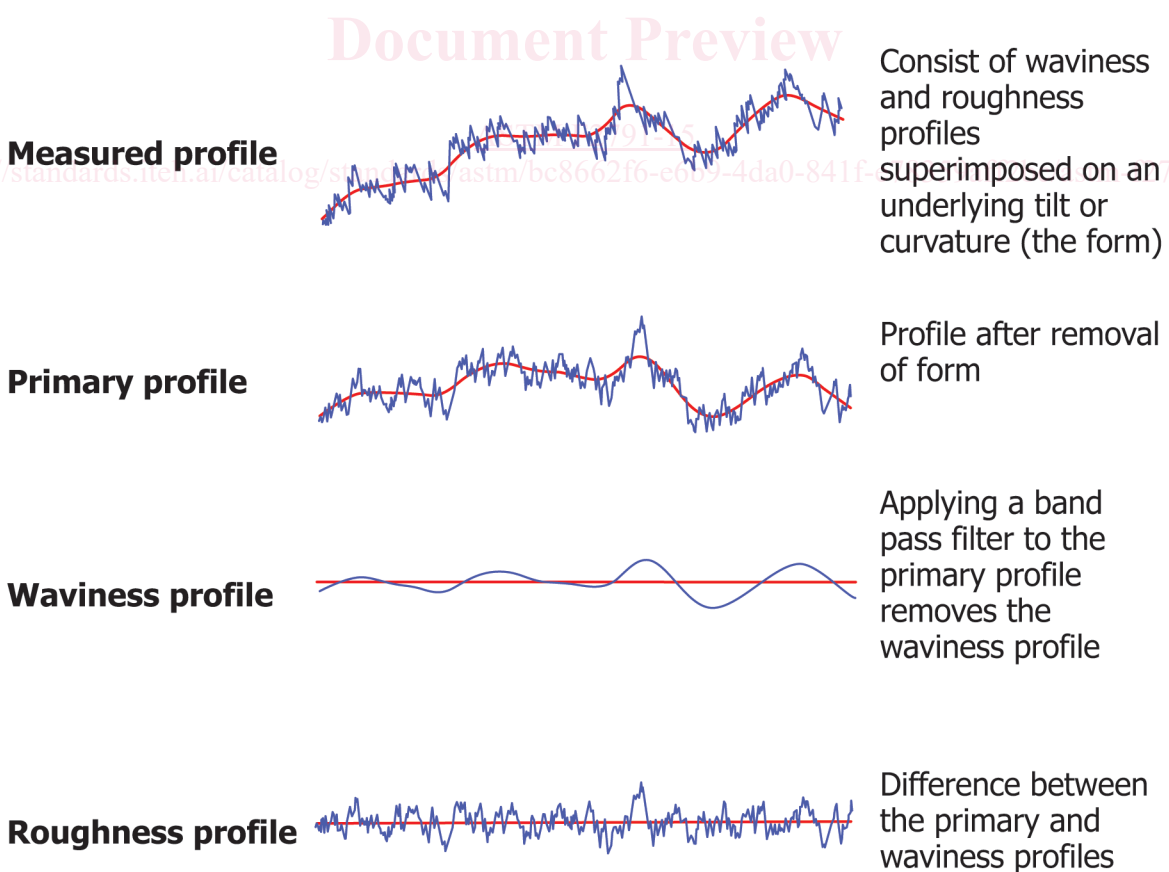
FIG. 2 Summary of Stages Involved in Analysis of Measured Profile to Obtain a Roughness Profile
