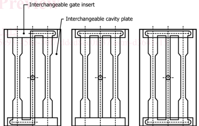
FIG. A1.2 Cavity and Runner Layout for Large Tensile Specimens
