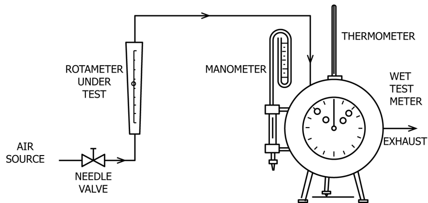
FIG. 1 Calibration Assembly Using Wet Test Meter
