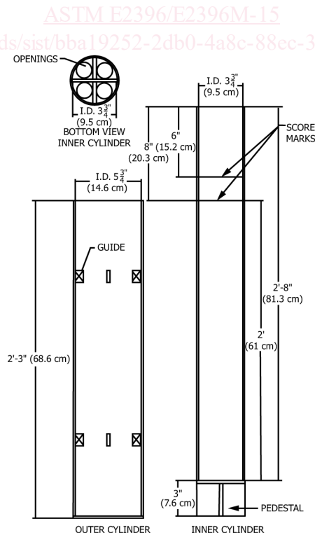
FIG. 1 Equipment Fabrication Detail
