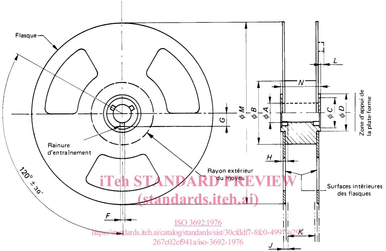
FIGURE 1 – Bobine
