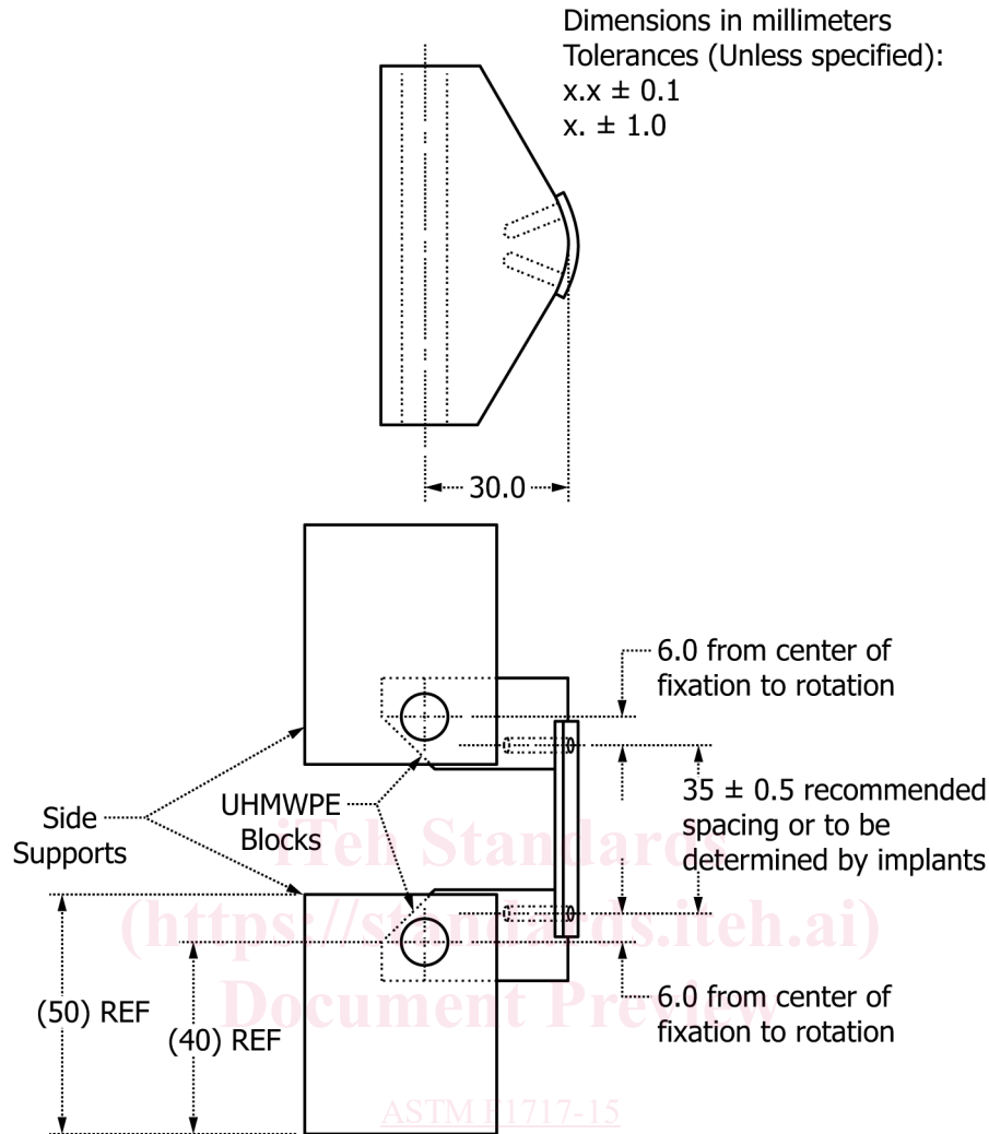
FIG. 4 Cervical Unilateral Construct Test Setup for Screws or Bolts for Plates
