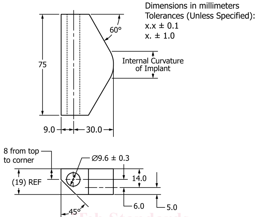
FIG. 5 Cervical Unilateral UHMWPE Block for Screws or Bolts Plates
