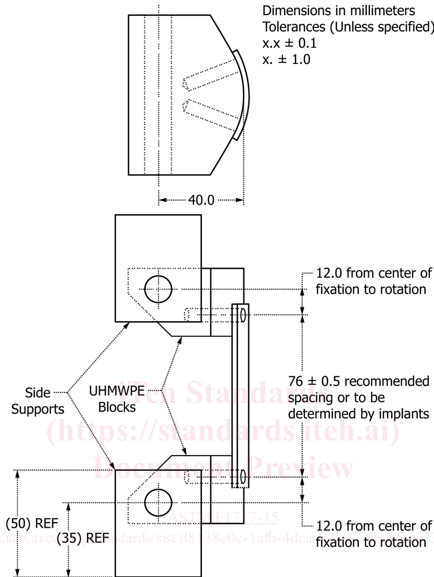
FIG. 10 Lumbar Unilateral UHMWPE Block for Screws or Belts Construct for Plates
