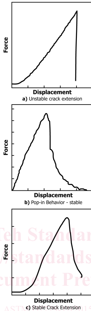
FIG. 2 Load-Displacement Behavior from Notched Beam Tests
