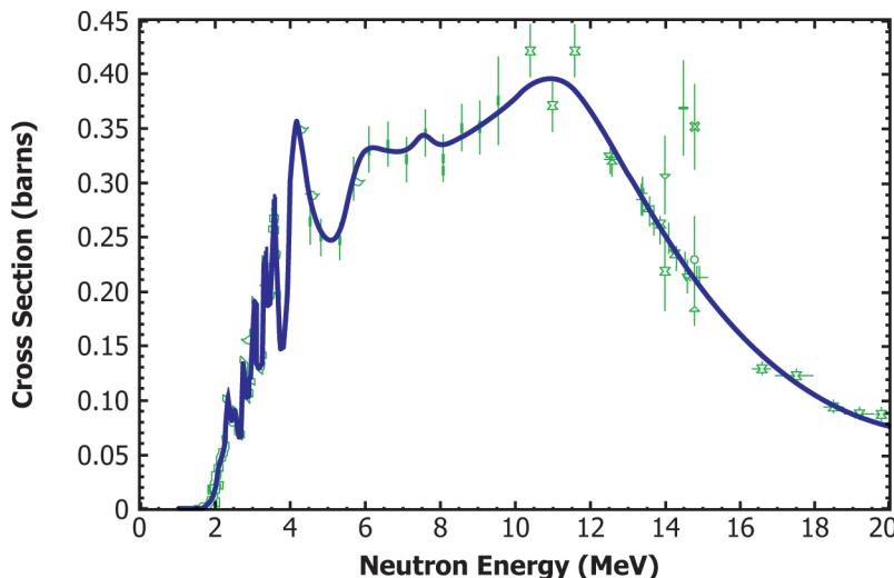
FIG. 1 32 S(n,p) 32 P Cross Section Versus Energy for the with EXFOR Experimental Data 32 S(n,p)( 32 3P) Reaction
