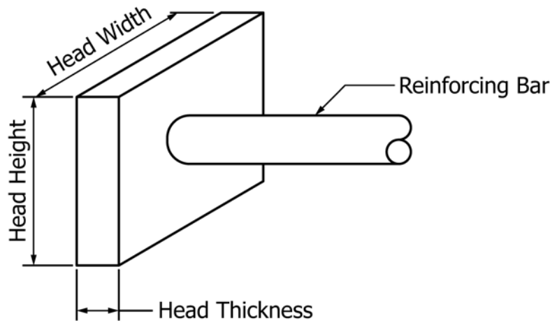
FIG. 1 Headed Reinforcing Bar
